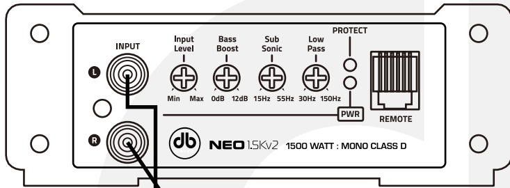
MONO SIGNAL CONNECTION
