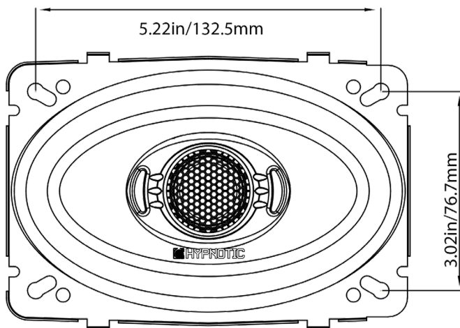
Mounting Template
