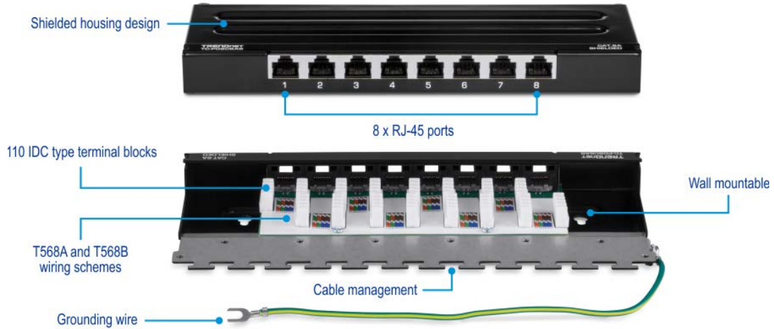
8-port Cat6A patch panel
