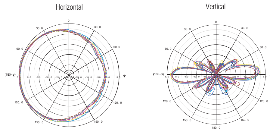
Radiation Pattern 5 GHz
